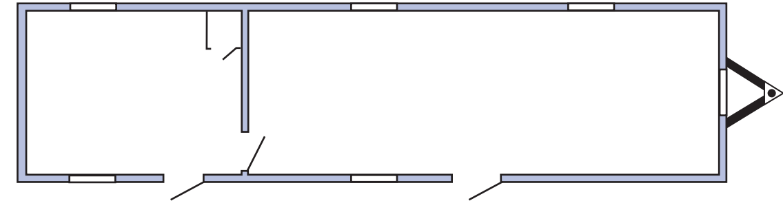
43' x 10' Two Rooms (also available in a 12' width)
