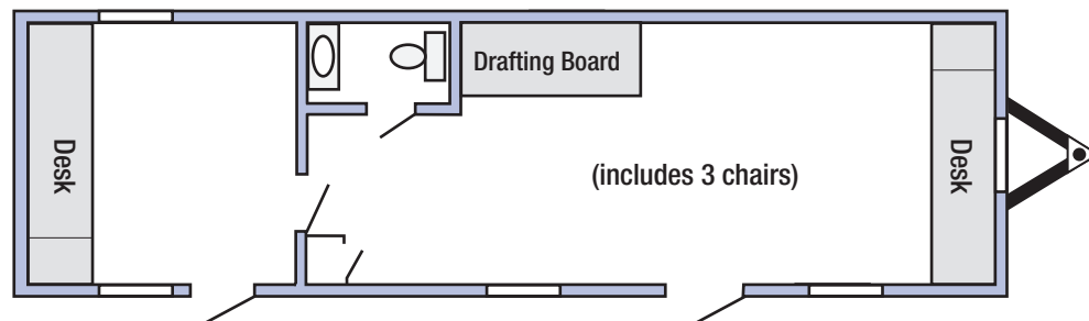
35' x 10' Two Rooms - 2 Desks, Drafting Board (washrooms optional)
