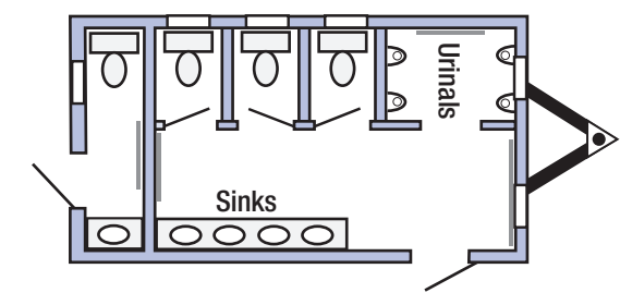
23' x 10' Wash Car No.2
